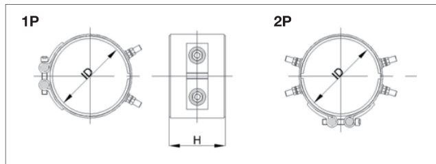
Band Heater
