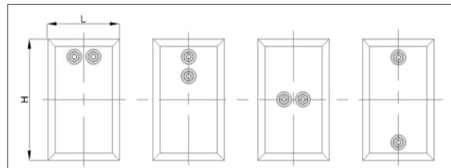
Strip Heater
