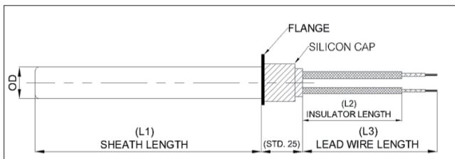
CARTRIDGE HEATER WITH FLANGE AND SILICON CAP
