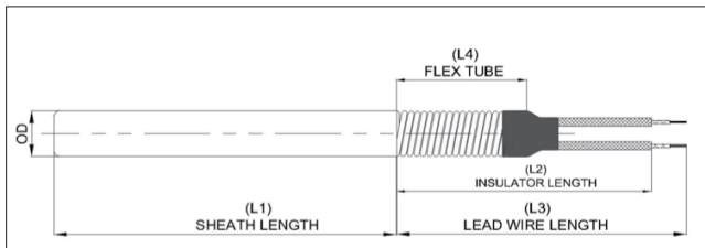
CARTRIDGE HEATER WITH FLEX TUBE
