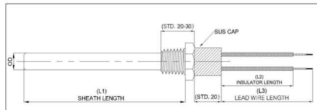
CARTRIDGE HEATER WITH SCREW
