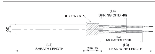
CARTRIDGE HEATER WITH SILICON CAP AND SPRING
