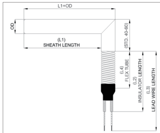
CARTRIDGE HEATER " L " SHAPE WITH FLEX TUBE
