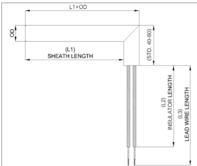
CARTRIDGE HEATER " L " SHAPE
